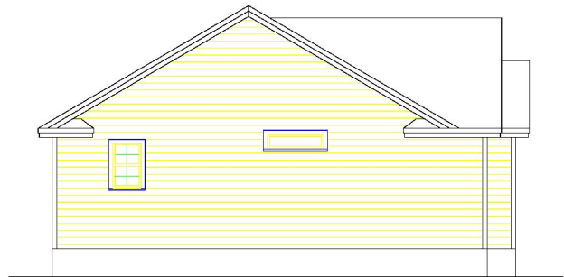
LEFT ELEVATION
